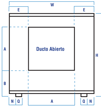
VISTA FRONTAL
